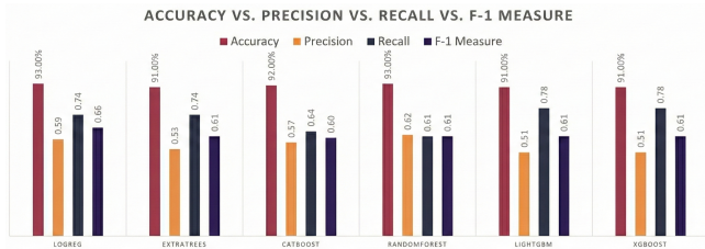
FIGURE 7. Bar charts of classification performance of supervised models tested for benchmark comparison.
