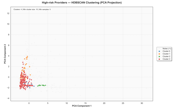
FIGURE 9. Two-dimensional PCA projection of standardized provider-level features for high-risk providers. Points are colored by HDBSCAN cluster label, with noise providers shown in grey.
