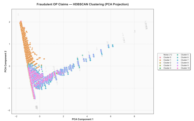
FIGURE 6. Two-dimensional PCA projections of standardized fraud-only claims, showing HDBSCAN clusters of fraudulent outpatient claims. Points are colored by cluster labels, with noise points shown in grey.
